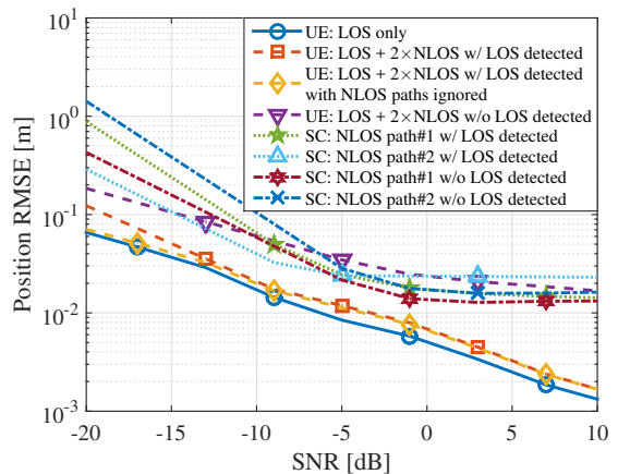
Fig. 5. Estimation RMSE for the UE and scatterer (SC) position by considering the LOS only and LOS+2×NLOS scenarios including distinct LOS detection information and handling of NLOS paths.
